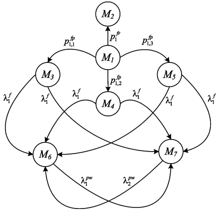
Fig. 8. Reachability graph of cyber-net (one-firewall-two-machines).
